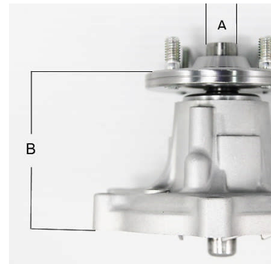
Measuring Points. A is shaft B is height
